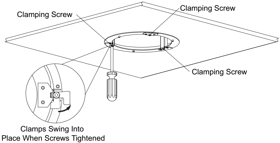
Figure: Indoor In-Ceiling Mount Installation
