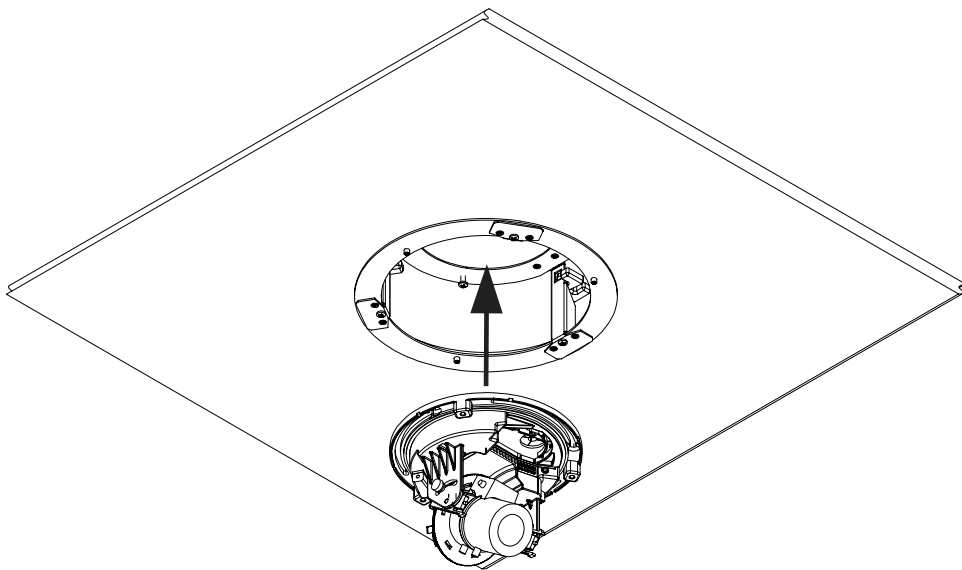
Figure: Dome Camera Installation
