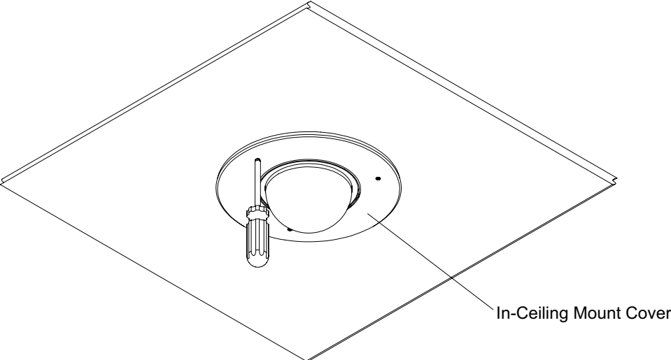
Figure: In-Ceiling Cover Installation
